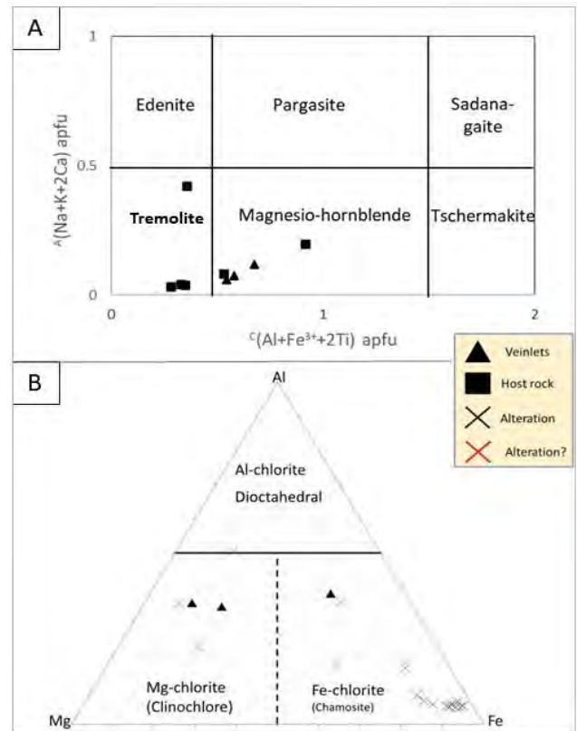
Figure 2 Compositions of amphibole and chlorite: A) Classification diagram of low aluminas amphiboles (after Hawthorne et al., 2012). B) Classification diagram of chlorites (after Zane & Weiss, 1998).
