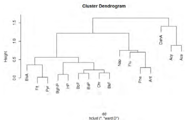
Fig. 2 Cluster dendrogram representing the relationships among the PAH compounds
